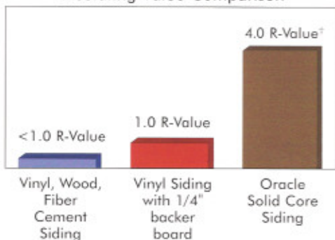
Insulating Value Comparison
